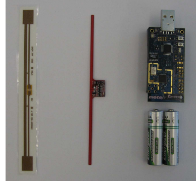
Figure 1 —Standard UHF Class 1 Gen 2 RFID tag, Intel WISP, Telos Mote
